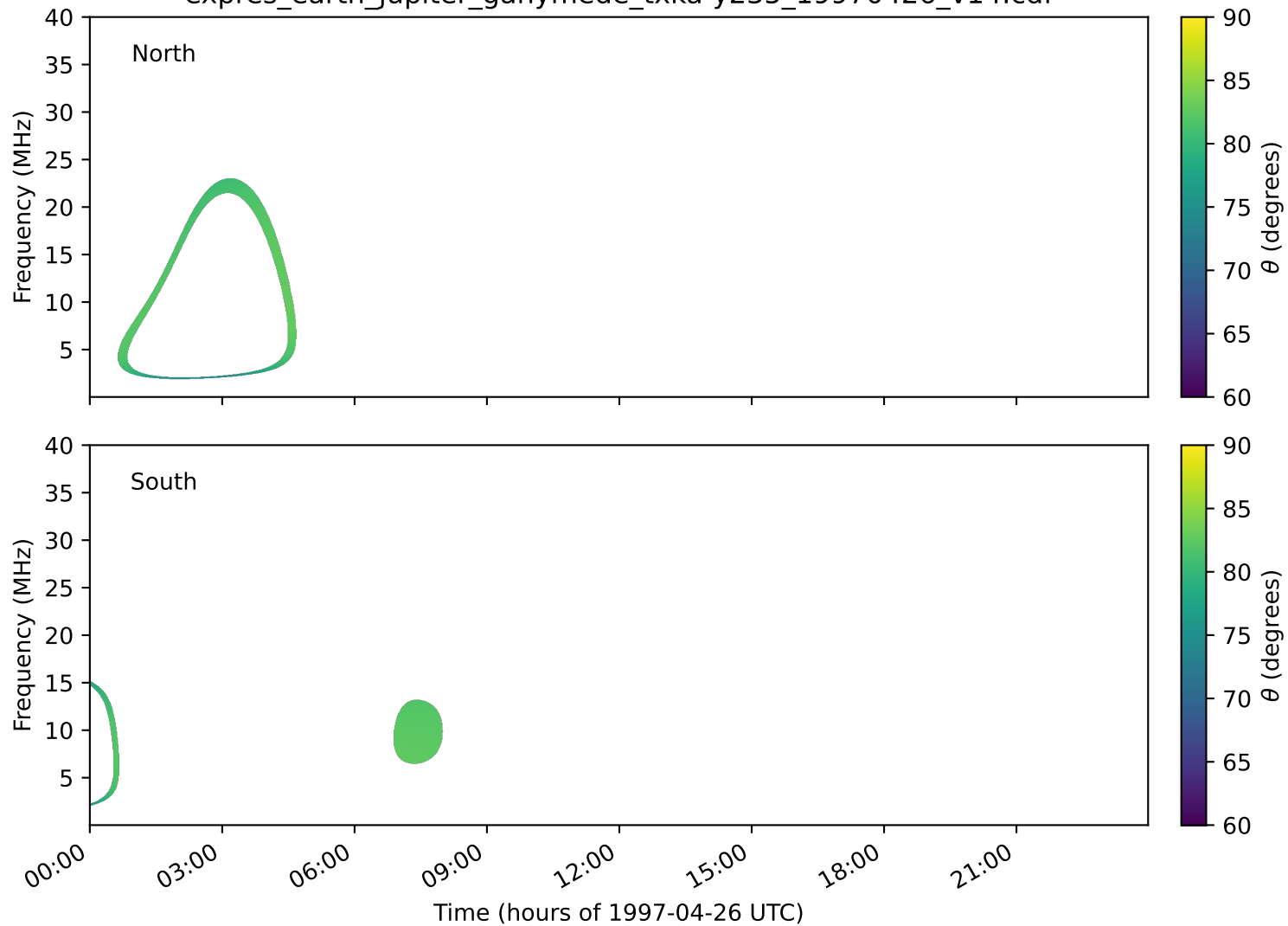
expres_earth_jupiter_ganymede_txka-y235_19970426_v14.cdf
