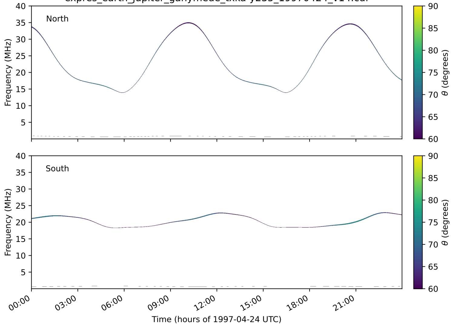
expres_earth_jupiter_ganymede_txka-y235_19970424_v14.cdf
