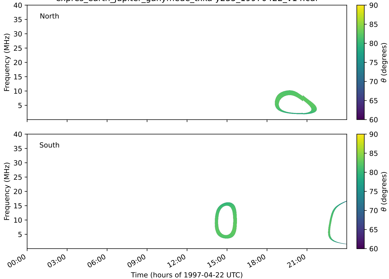
expres_earth_jupiter_ganymede_txka-y235_19970422_v14.cdf
