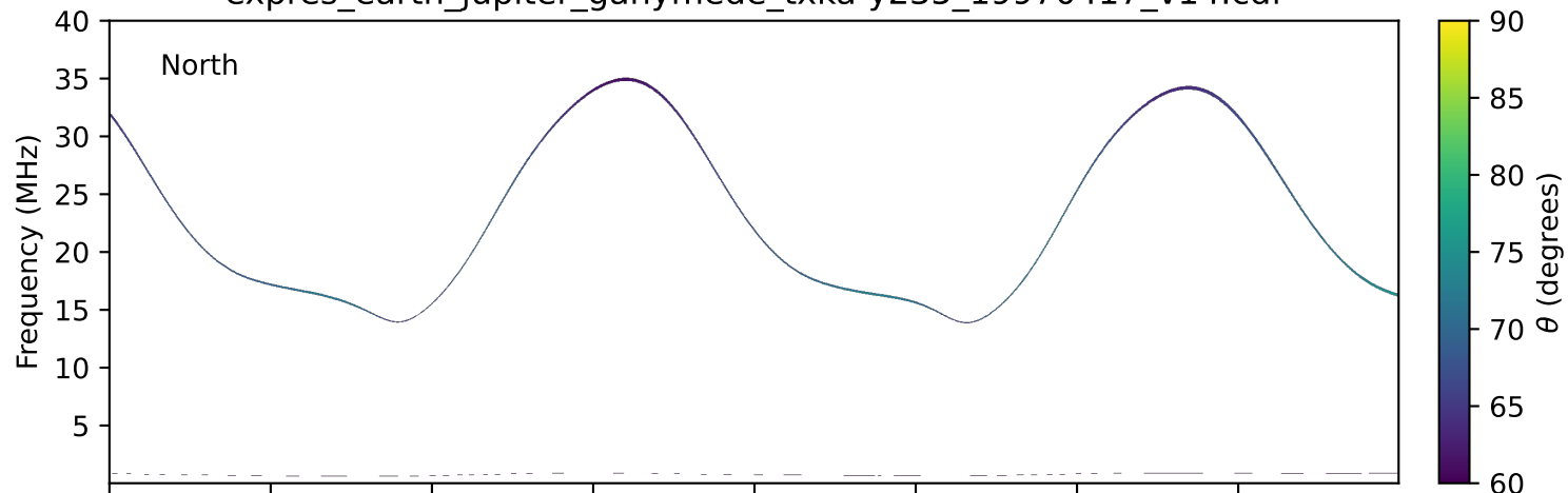
expres_earth_jupiter_ganymede_txka-y235_19970417_v14.cdf
