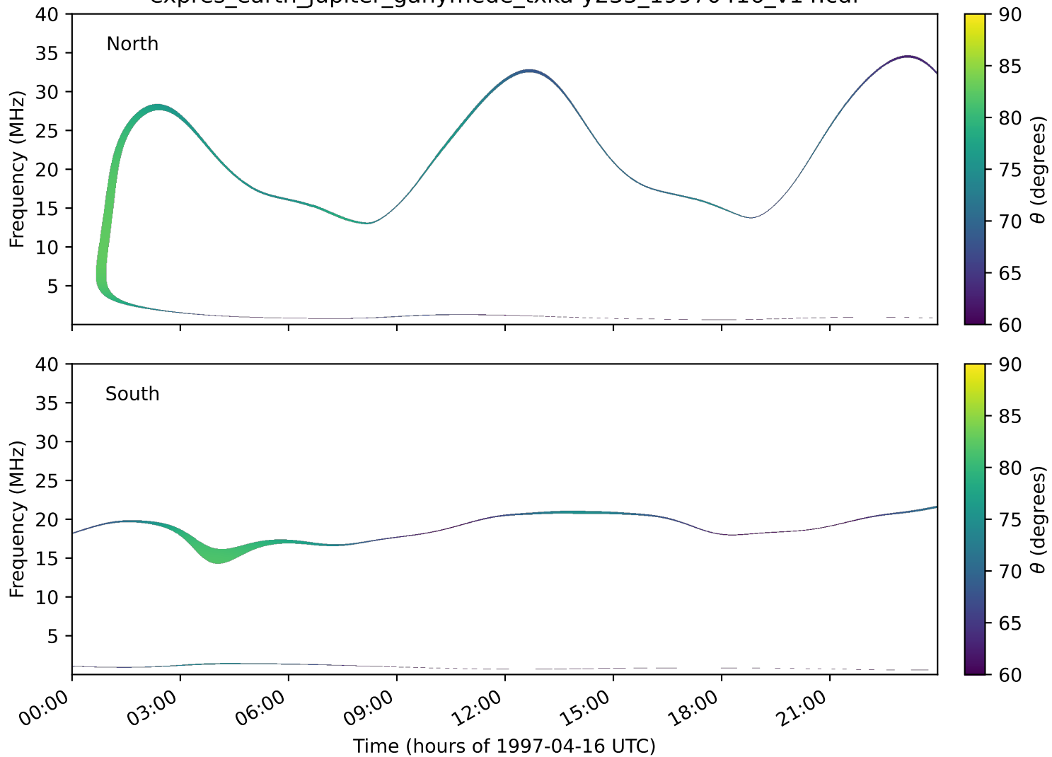
expres_earth_jupiter_ganymede_txka-y235_19970416_v14.cdf
