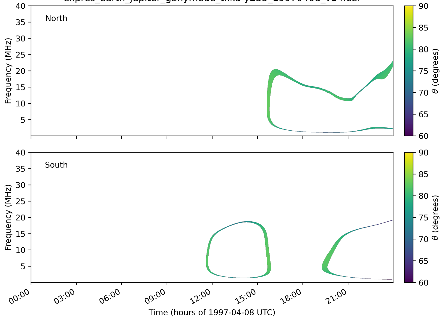
expres_earth_jupiter_ganymede_txka-y235_19970408_v14.cdf
