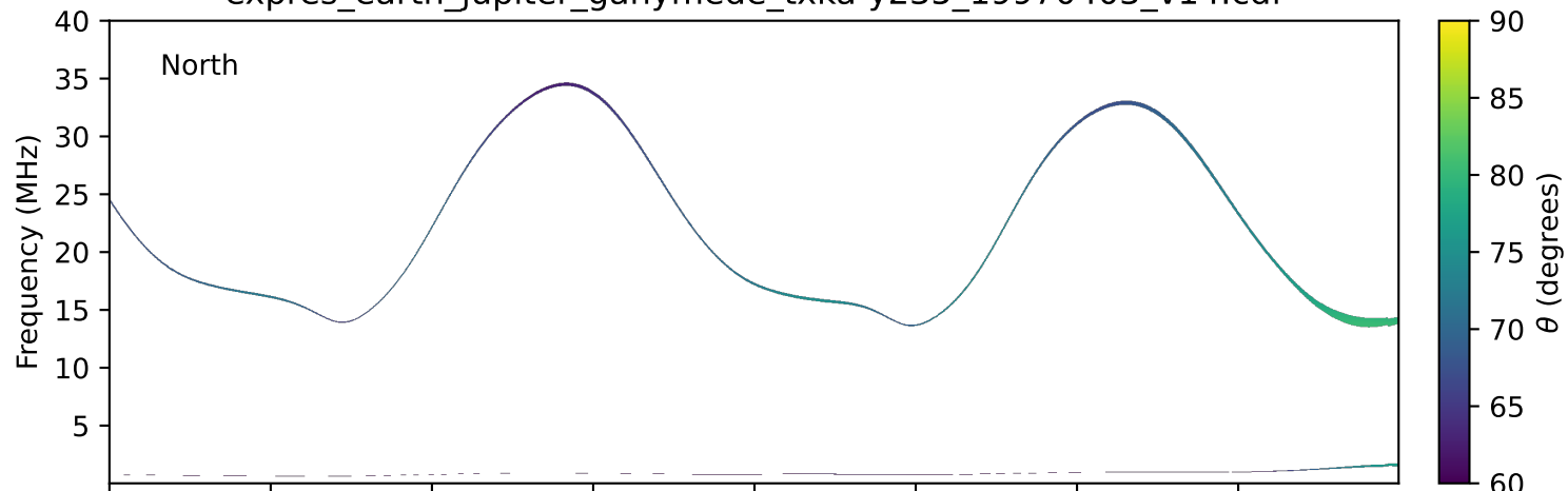
expres_earth_jupiter_ganymede_txka-y235_19970403_v14.cdf
