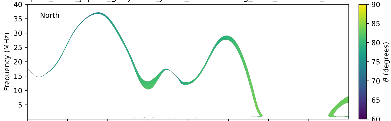
expres_earth_jupiter_ganymede_jrm33_lossc-wid1deg_3kev_19970404_v11.cdf
