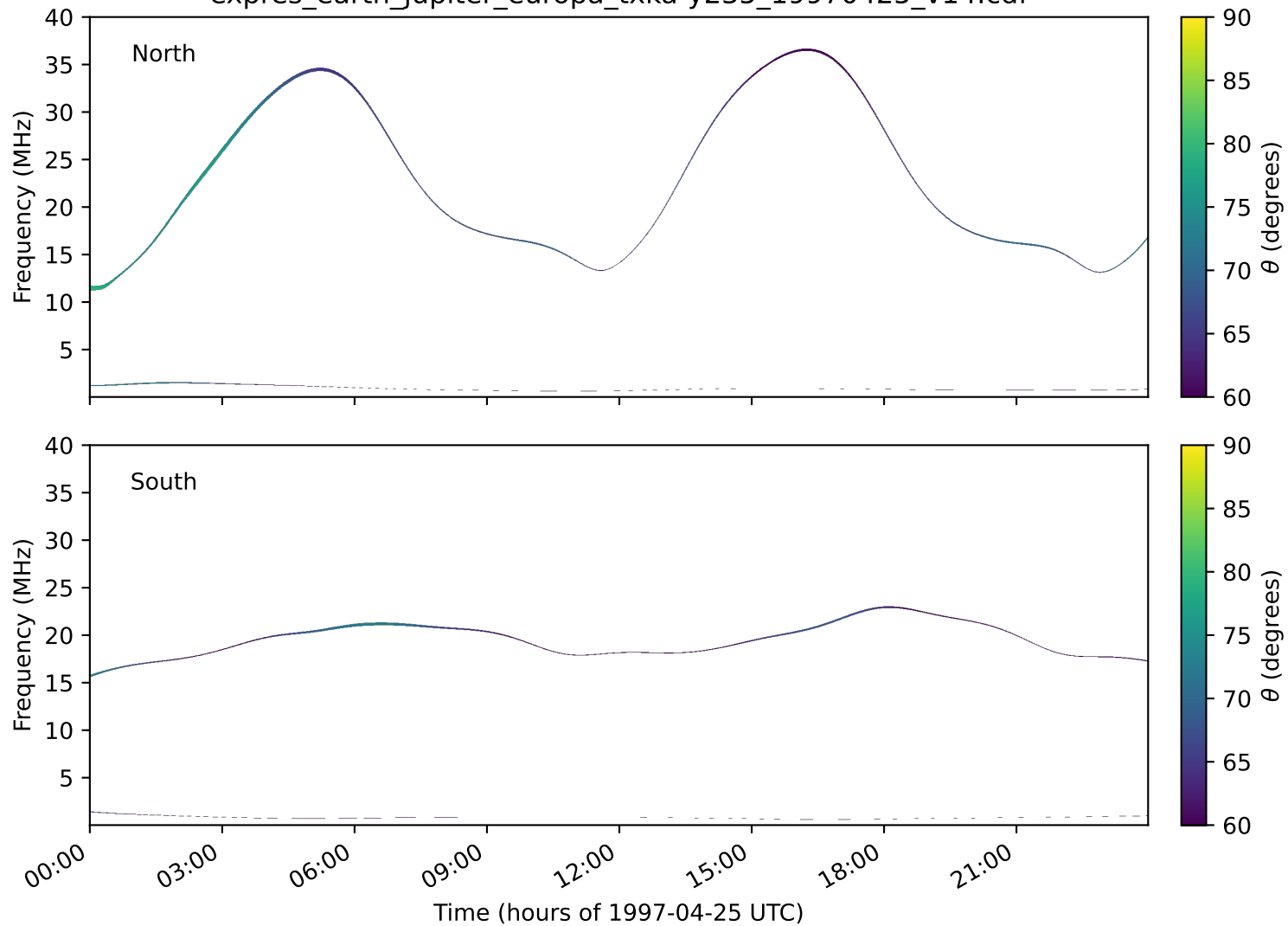
expres_earth_jupiter_europa_txka-y235_19970425_v14.cdf
