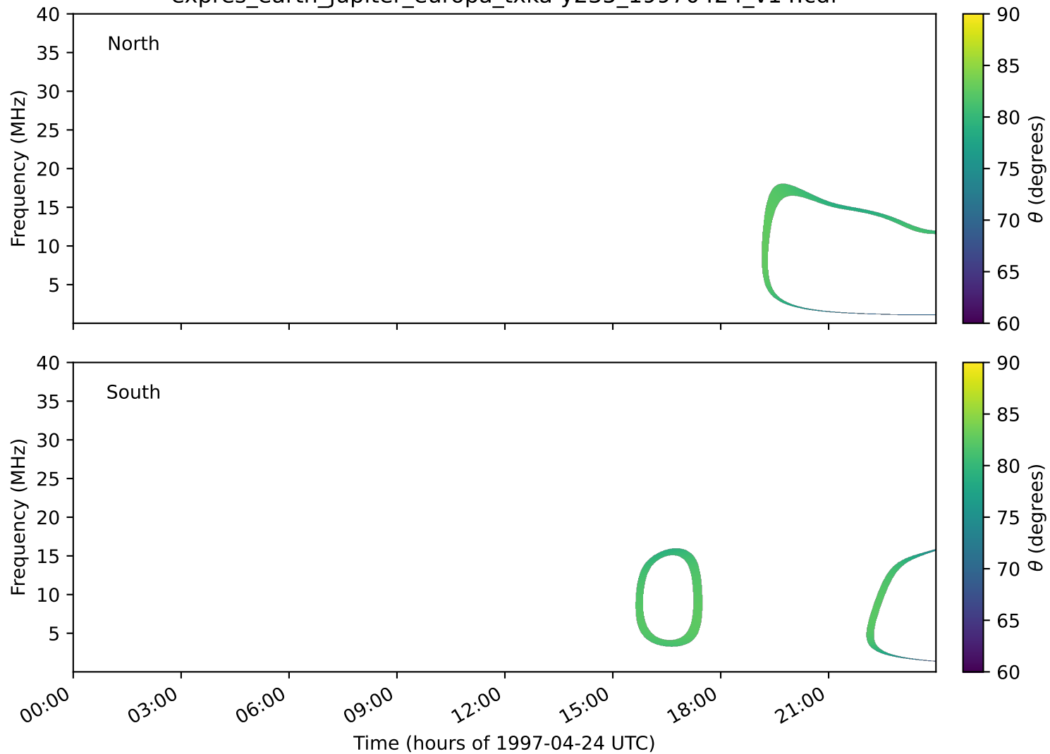
expres_earth_jupiter_europa_txka-y235_19970424_v14.cdf
