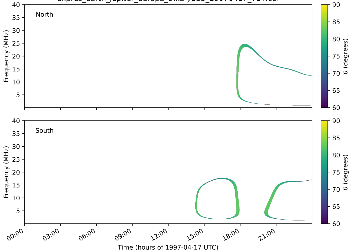
expres_earth_jupiter_europa_txka-y235_19970417_v14.cdf
