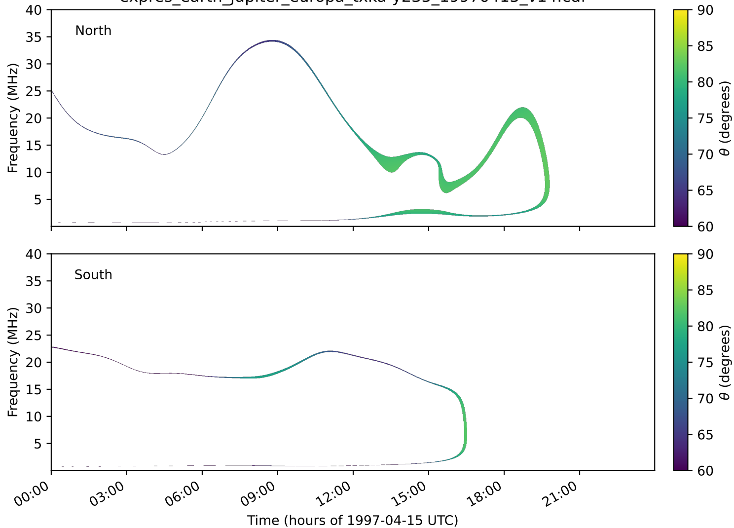
expres_earth_jupiter_europa_txka-y235_19970415_v14.cdf
