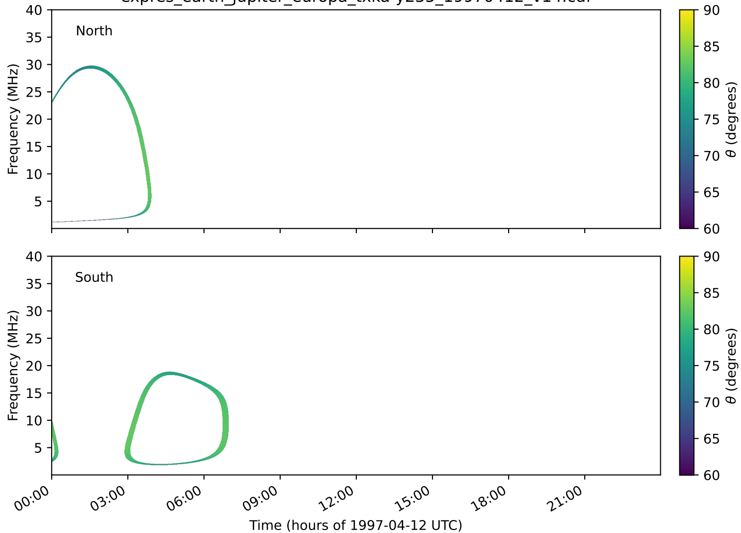
expres_earth_jupiter_europa_txka-y235_19970412_v14.cdf
