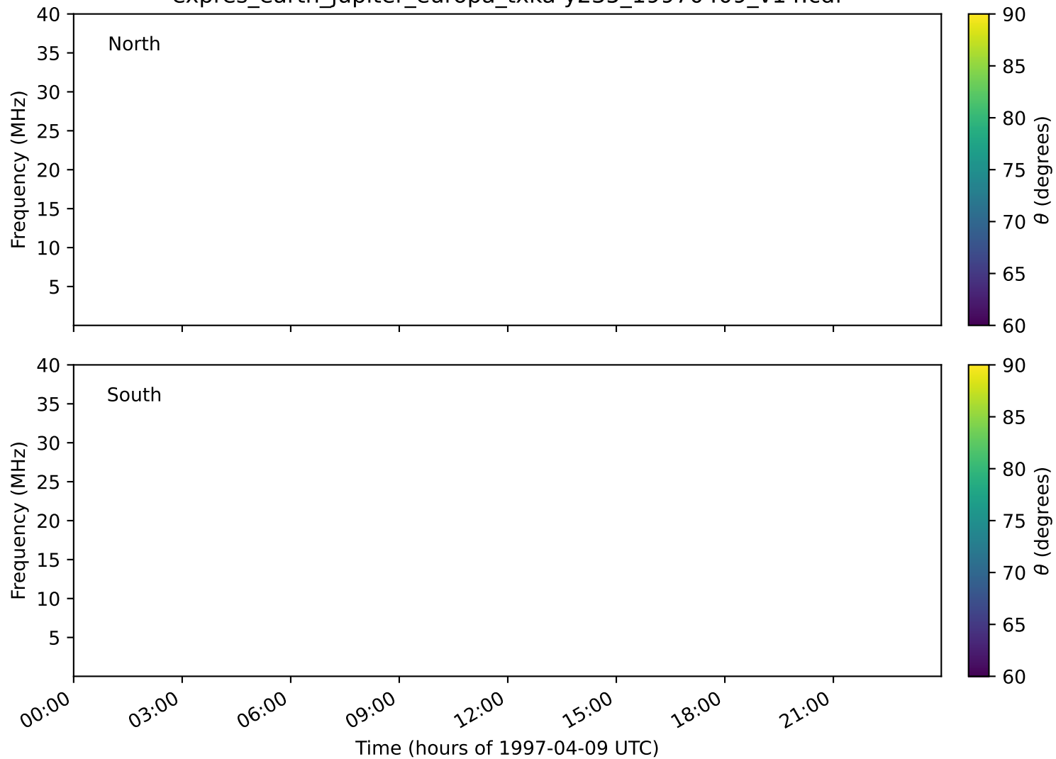
expres_earth_jupiter_europa_txka-y235_19970409_v14.cdf
