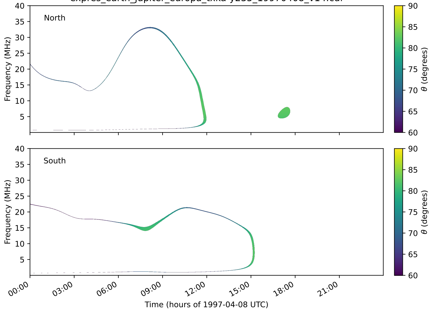
expres_earth_jupiter_europa_txka-y235_19970408_v14.cdf
