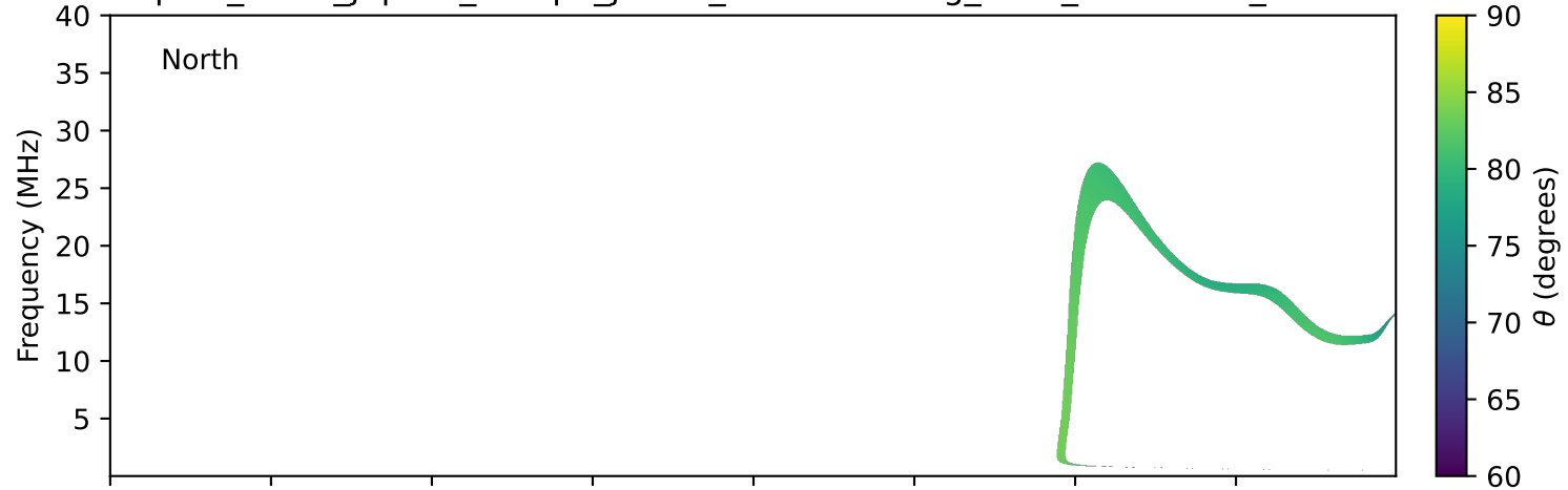
expres_earth_jupiter_europa_jrm33_lossc-wid1deg_3kev_19970417_v11.cdf
