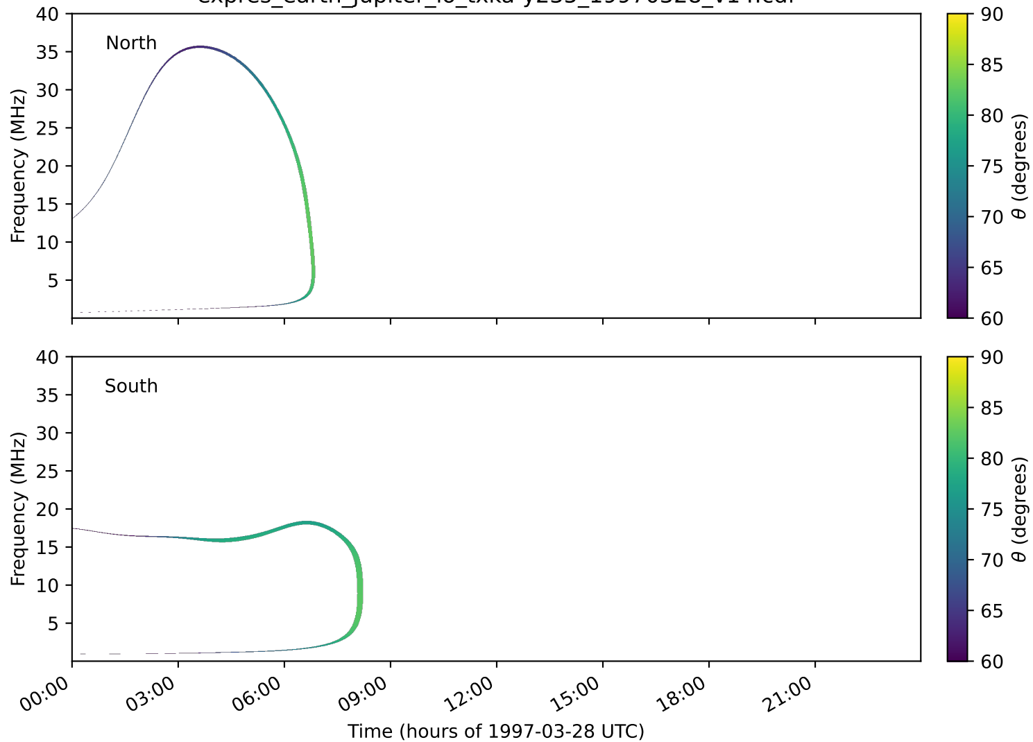
expres_earth_jupiter_io_txka-y235_19970328_v14.cdf
