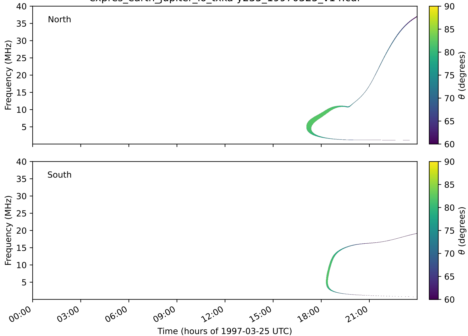
expres_earth_jupiter_io_txka-y235_19970325_v14.cdf
