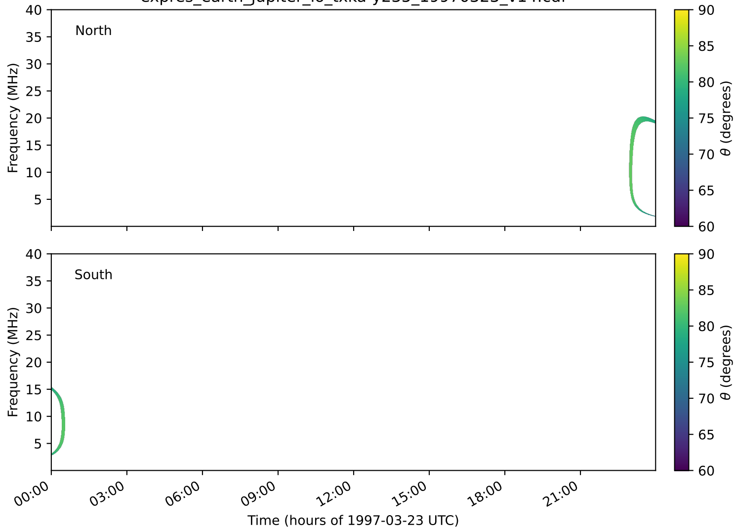
expres_earth_jupiter_io_txka-y235_19970323_v14.cdf
