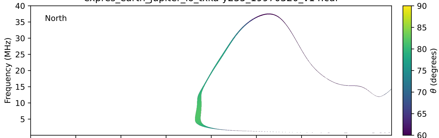
expres_earth_jupiter_io_txka-y235_19970320_v14.cdf
