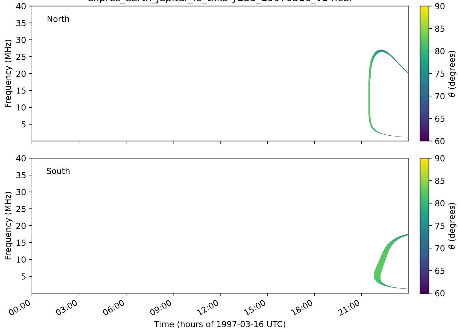
expres_earth_jupiter_io_txka-y235_19970316_v14.cdf
