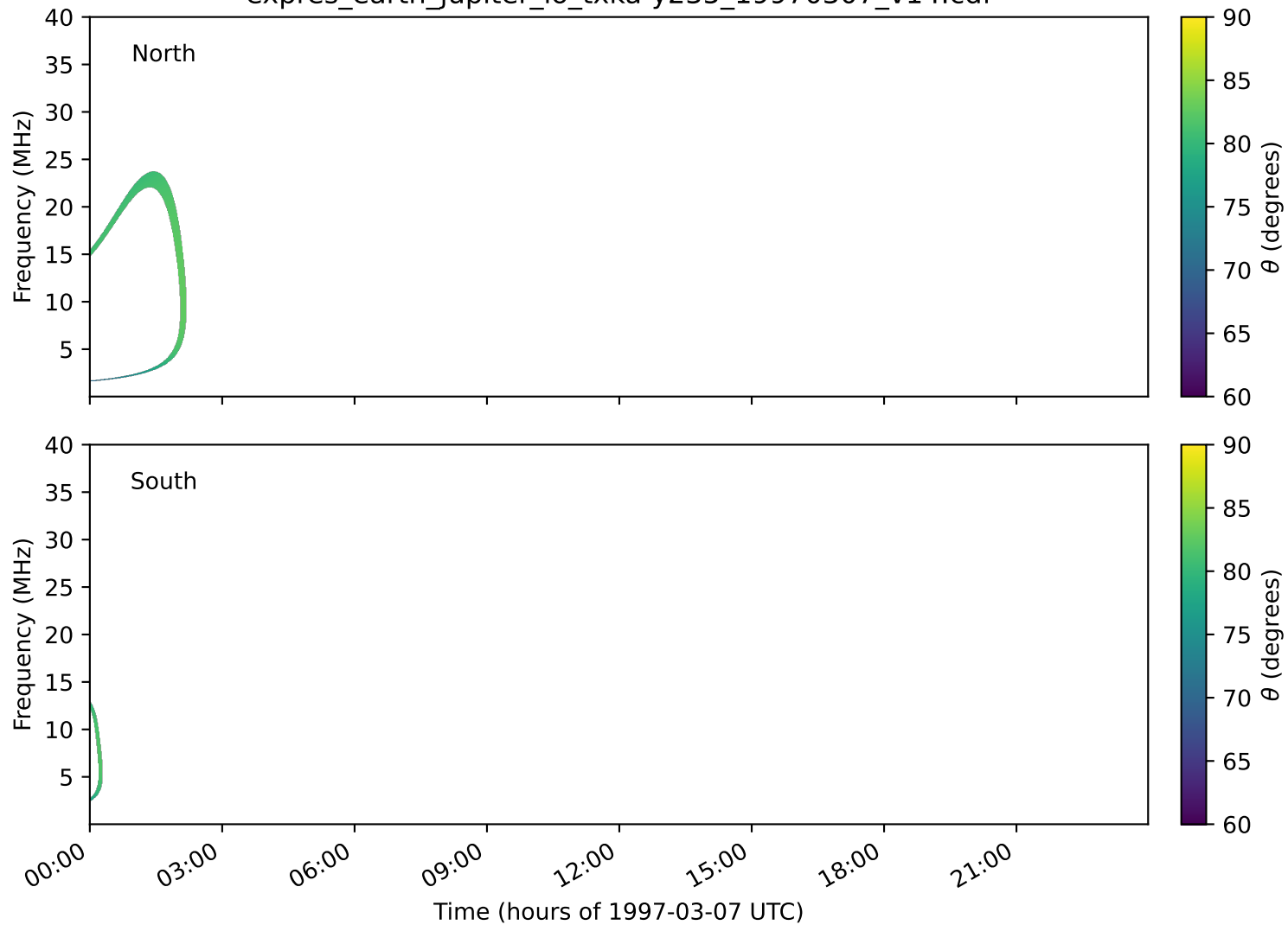
expres_earth_jupiter_io_txka-y235_19970307_v14.cdf
