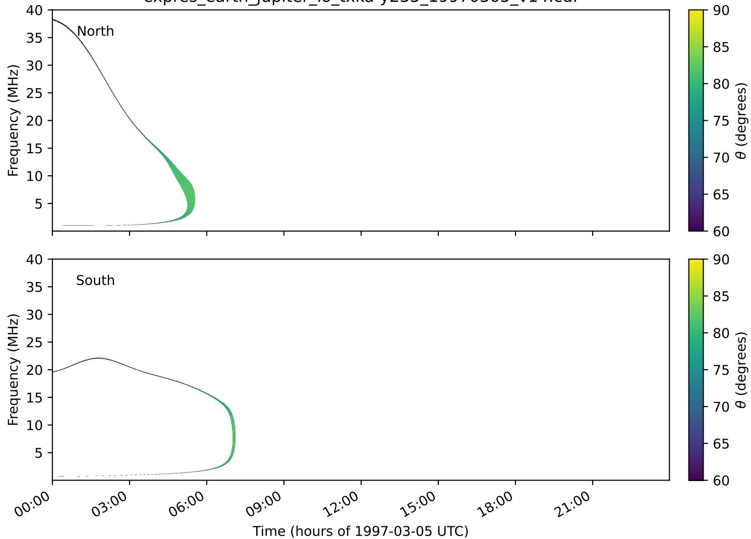
expres_earth_jupiter_io_txka-y235_19970305_v14.cdf
