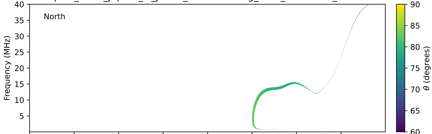
expres_earth_jupiter_io_jrm33_lossc-wid1deg_3kev_19970318_v11.cdf
