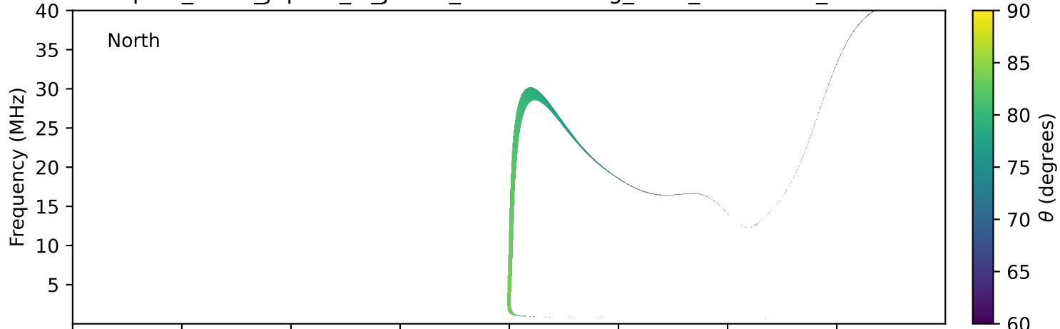
expres_earth_jupiter_io_jrm33_lossc-wid1deg_3kev_19970304_v11.cdf
