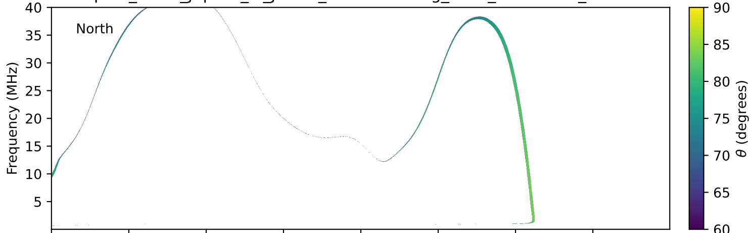
expres_earth_jupiter_io_jrm33_lossc-wid1deg_3kev_19970301_v11.cdf
