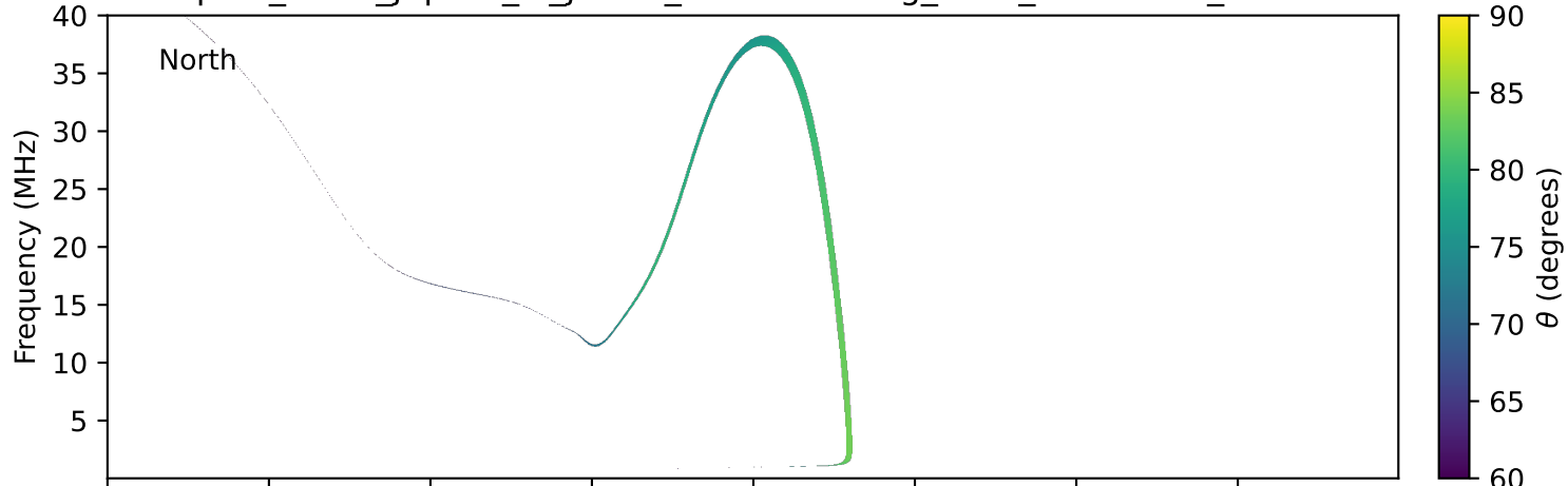
expres_earth_jupiter_io_jrm09_lossc-wid1deg_3kev_19970326_v11.cdf
