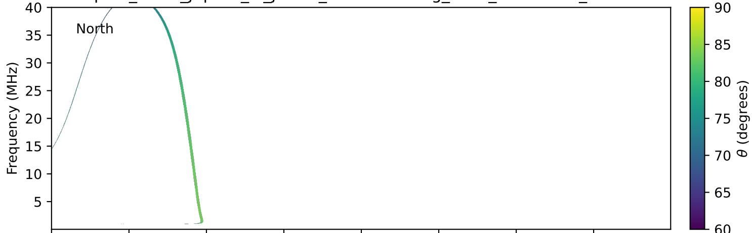
expres_earth_jupiter_io_jrm09_lossc-wid1deg_3kev_19970321_v11.cdf
