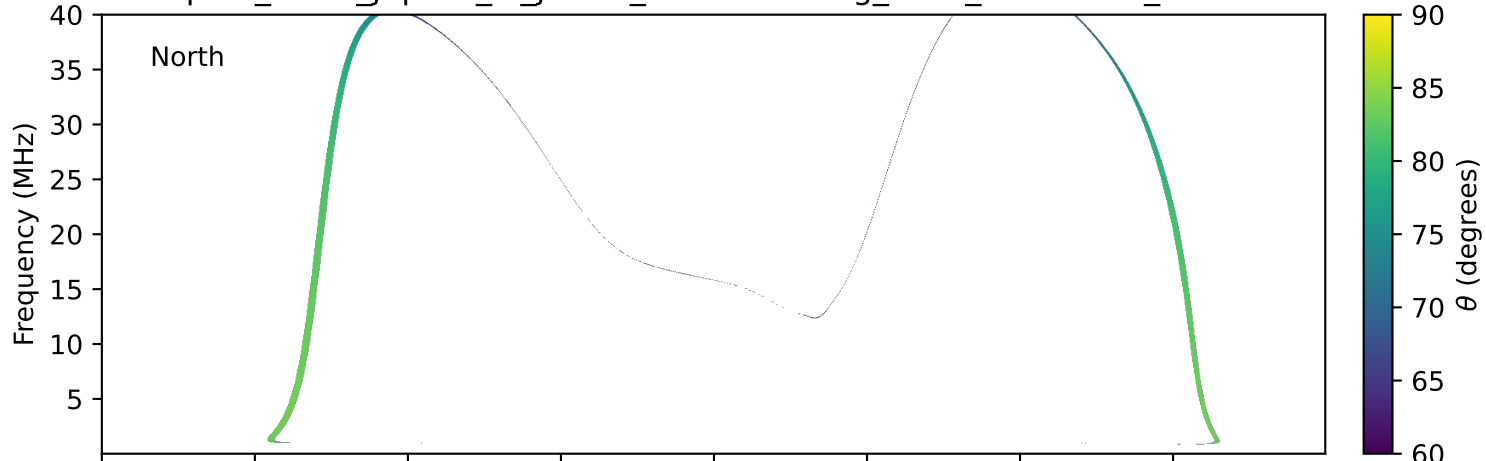
expres_earth_jupiter_io_jrm09_lossc-wid1deg_3kev_19970315_v11.cdf
