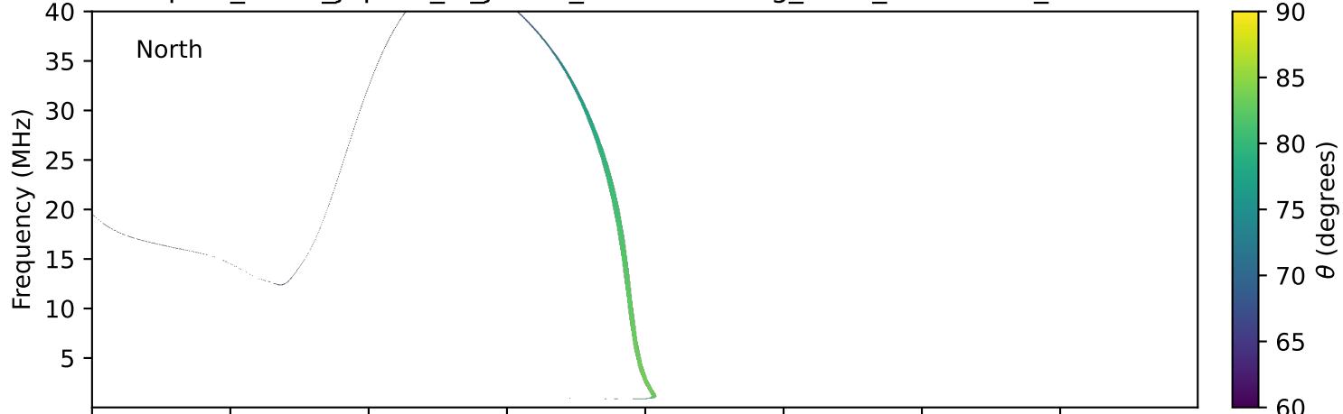
expres_earth_jupiter_io_jrm09_lossc-wid1deg_3kev_19970303_v11.cdf
