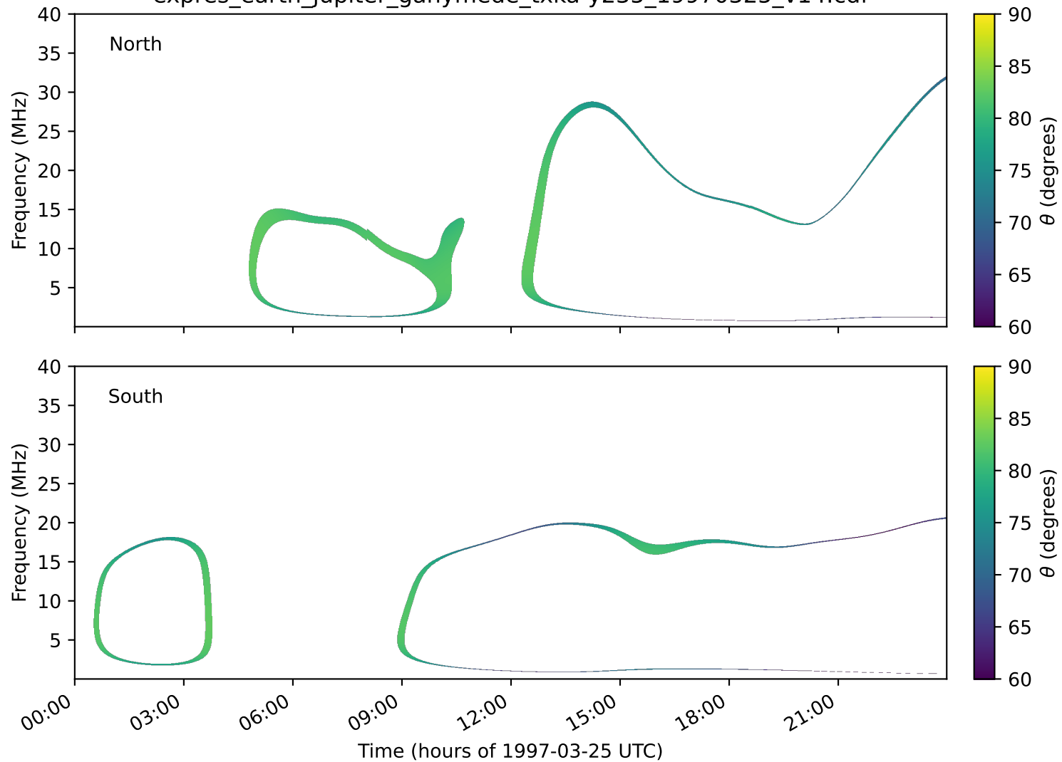
expres_earth_jupiter_ganymede_txka-y235_19970325_v14.cdf
