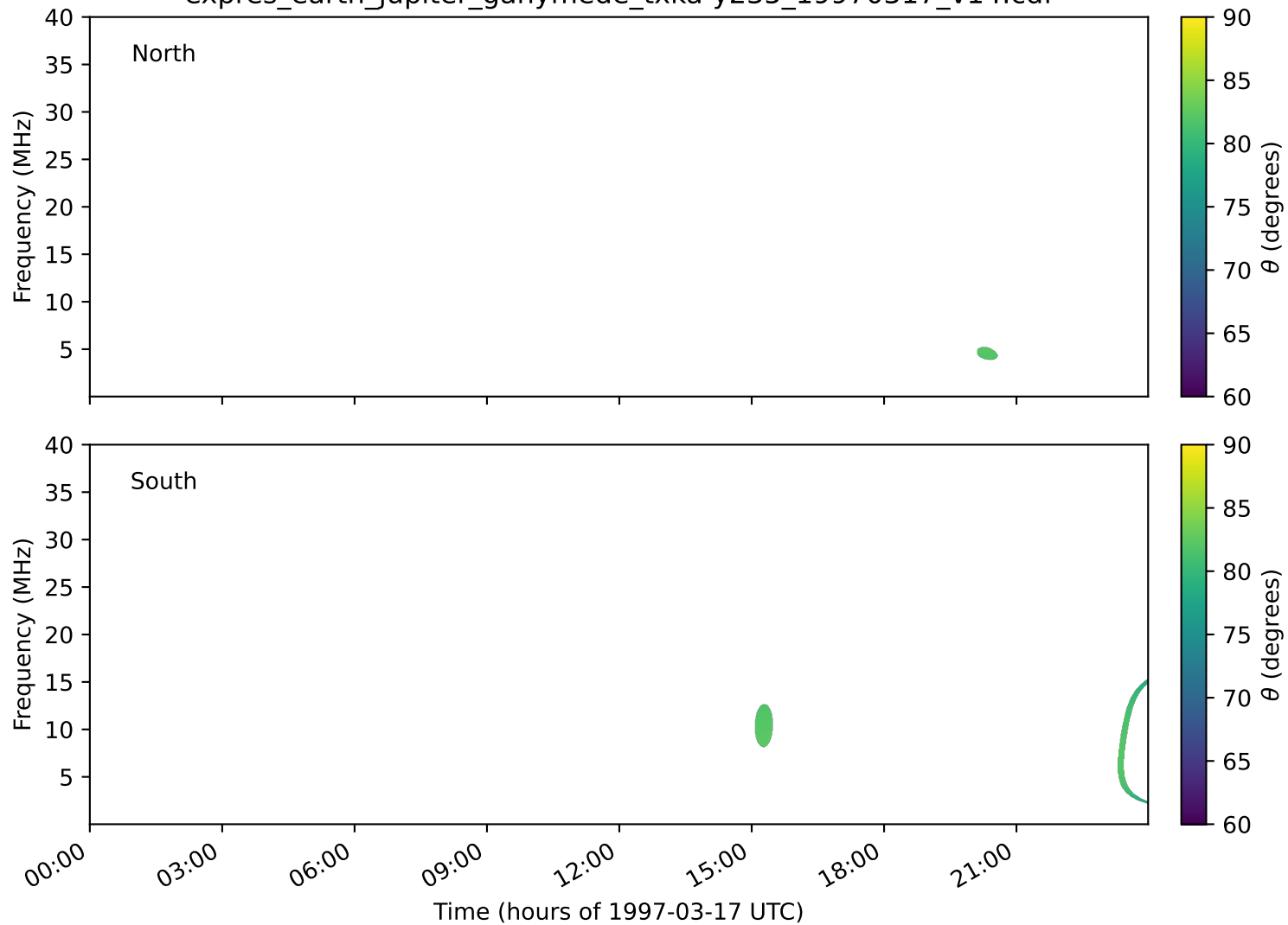
expres_earth_jupiter_ganymede_txka-y235_19970317_v14.cdf
