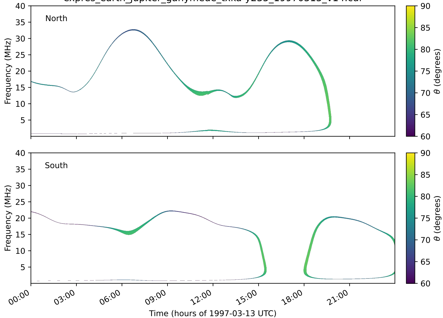
expres_earth_jupiter_ganymede_txka-y235_19970313_v14.cdf
