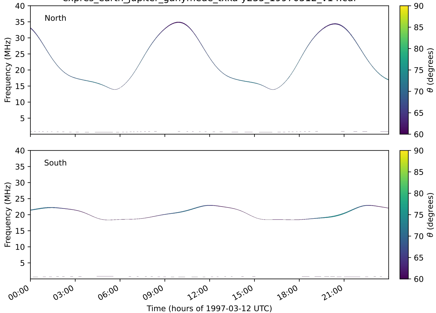
expres_earth_jupiter_ganymede_txka-y235_19970312_v14.cdf
