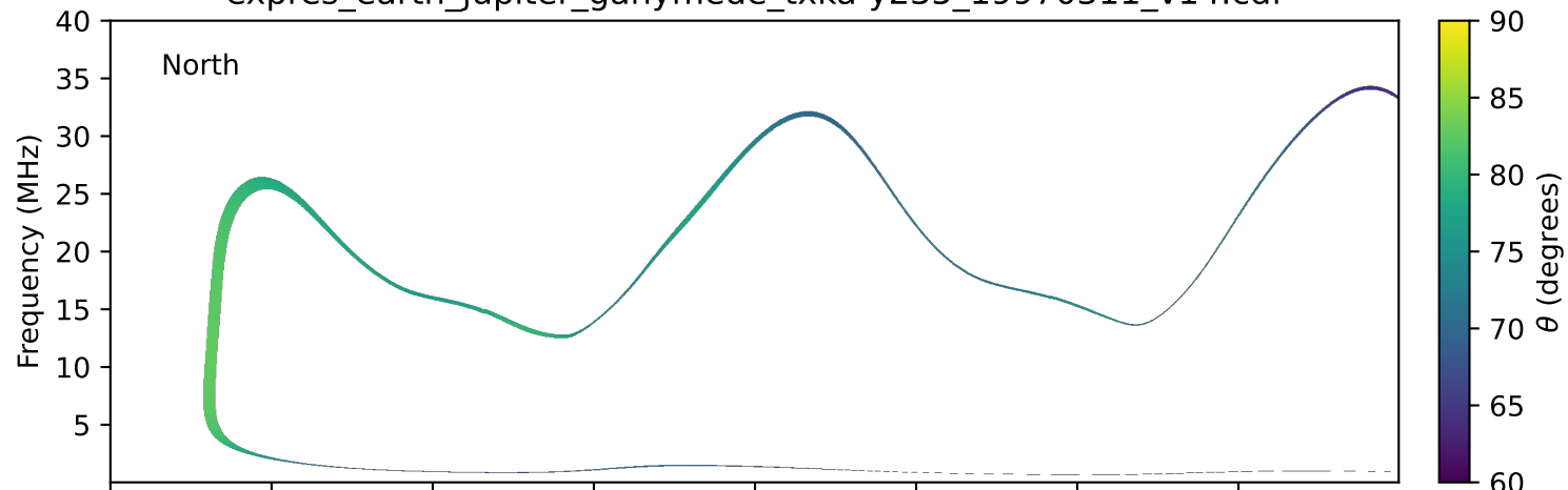
expres_earth_jupiter_ganymede_txka-y235_19970311_v14.cdf
