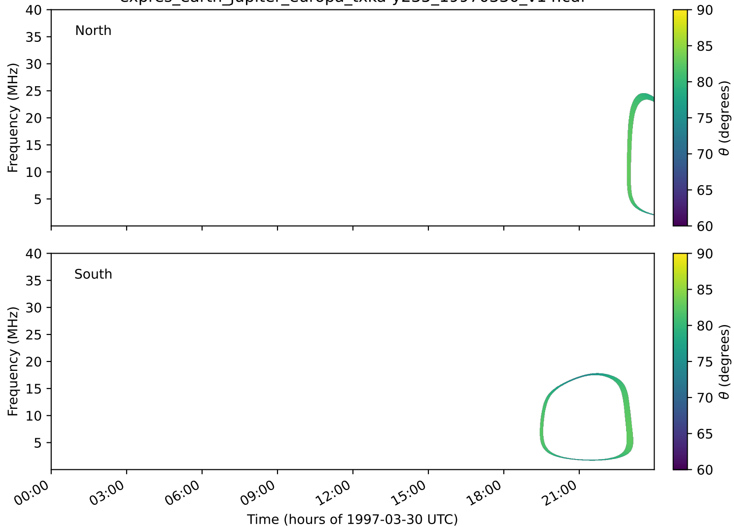
expres_earth_jupiter_europa_txka-y235_19970330_v14.cdf
