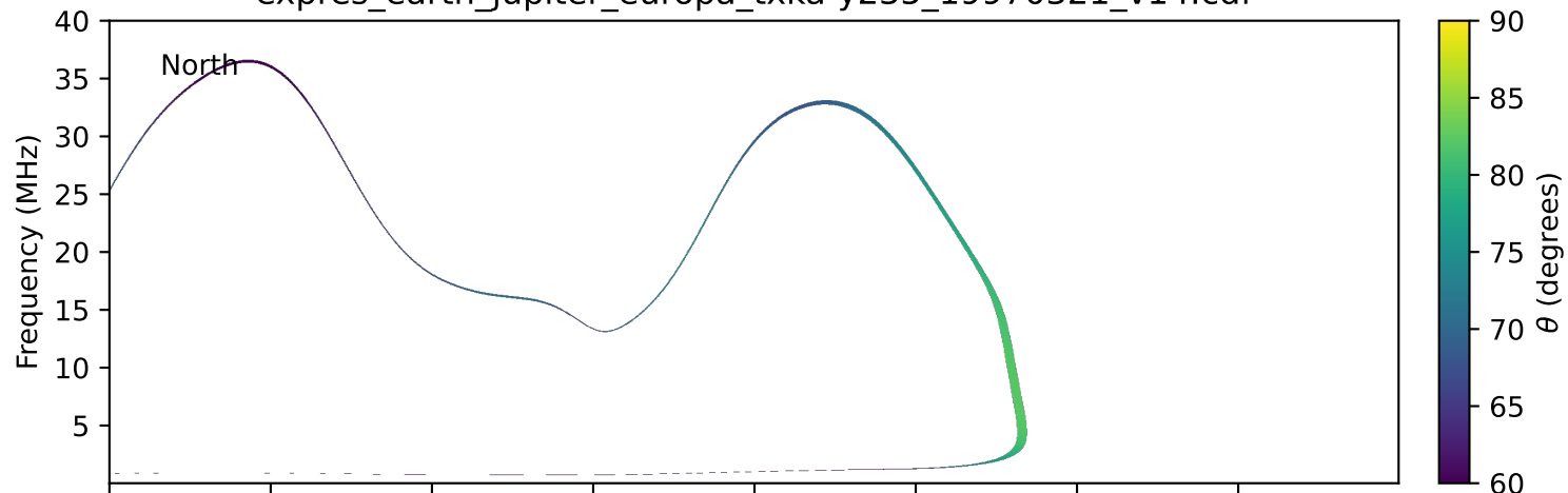
expres_earth_jupiter_europa_txka-y235_19970321_v14.cdf
