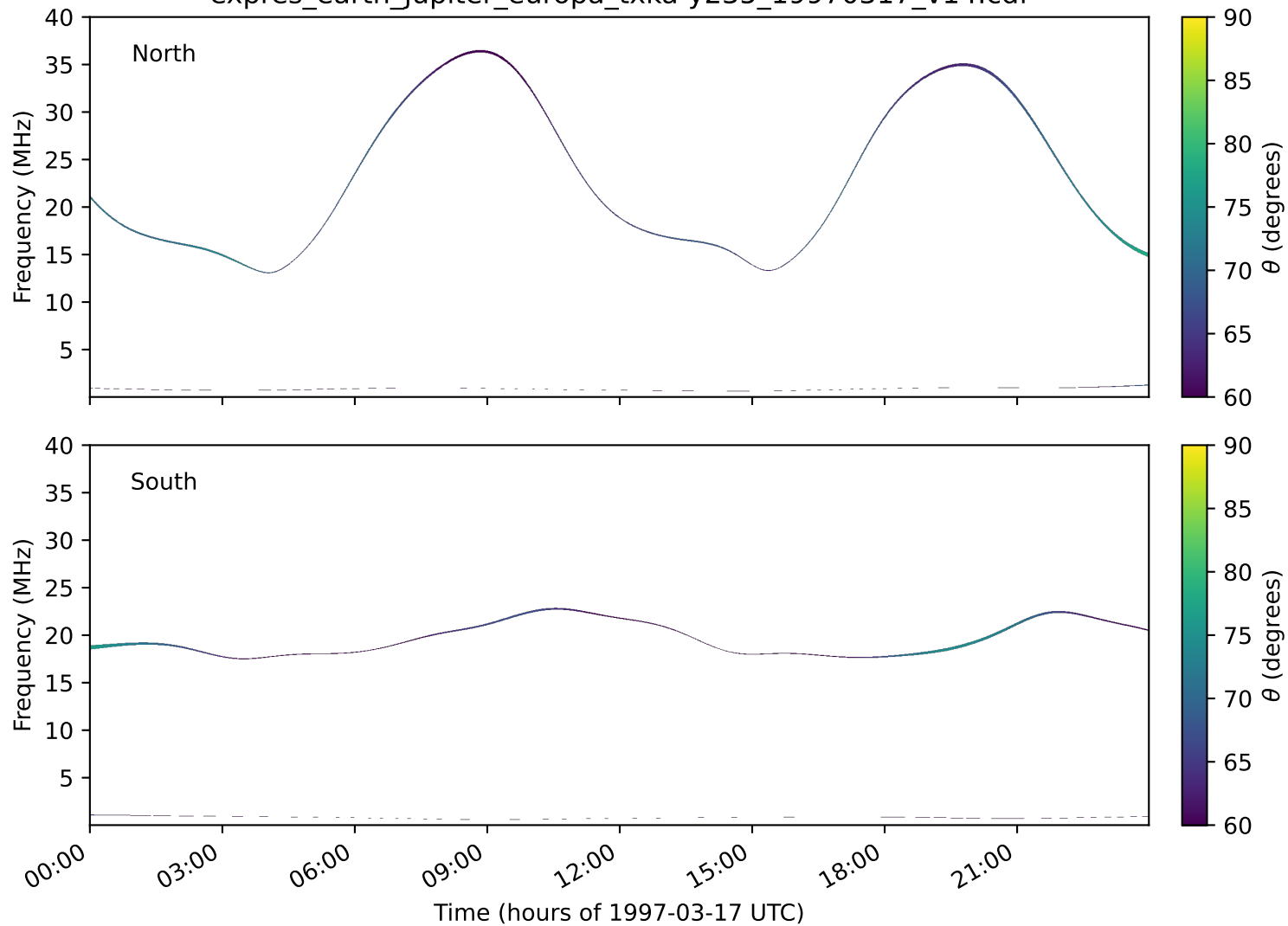
expres_earth_jupiter_europa_txka-y235_19970317_v14.cdf
