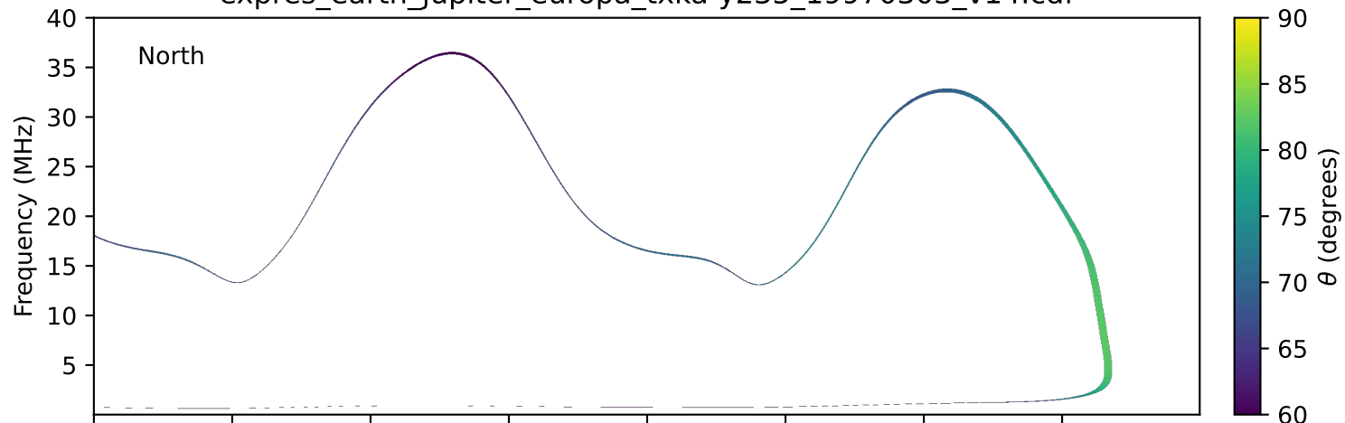
expres_earth_jupiter_europa_txka-y235_19970303_v14.cdf
