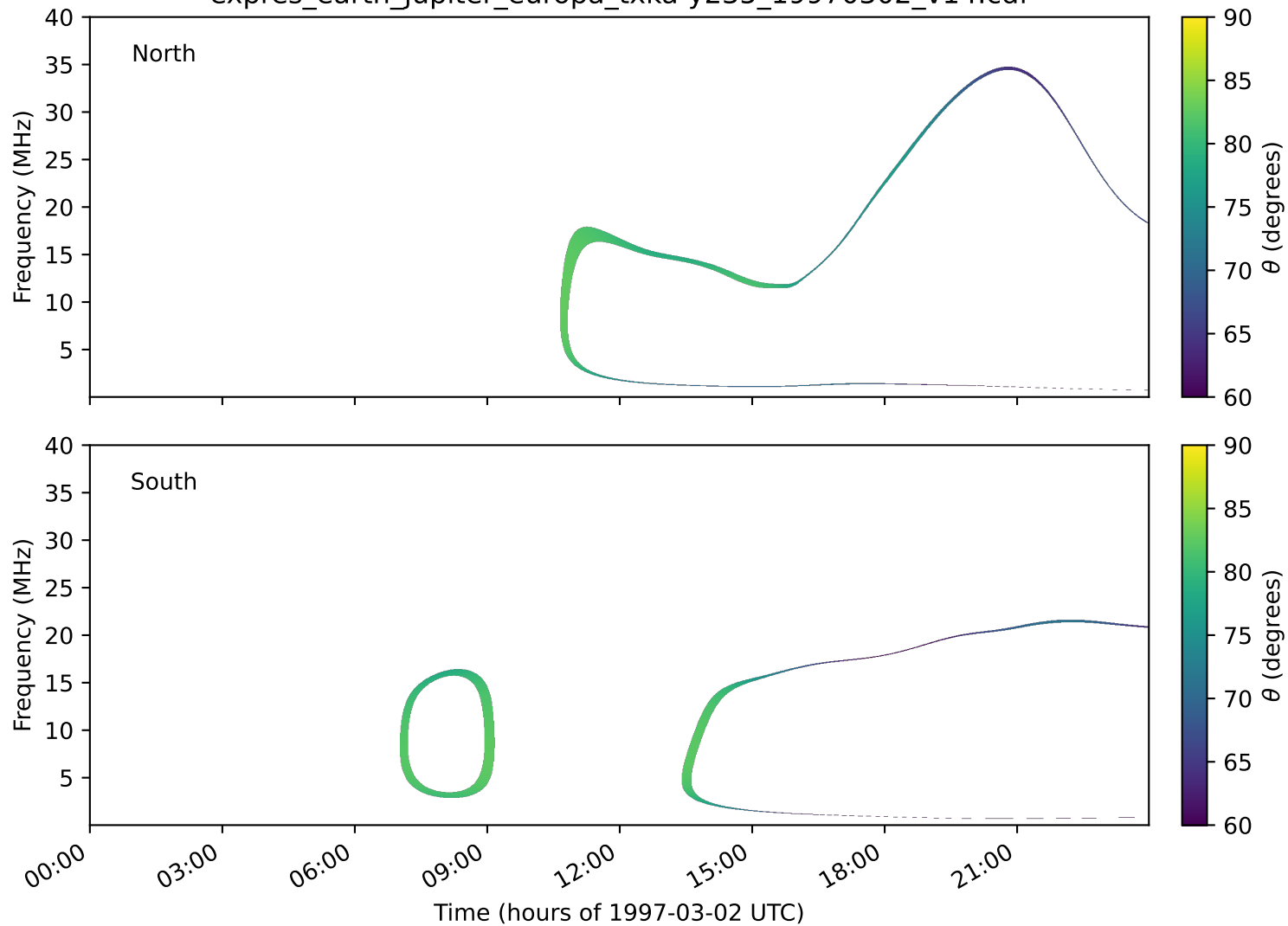
expres_earth_jupiter_europa_txka-y235_19970302_v14.cdf
