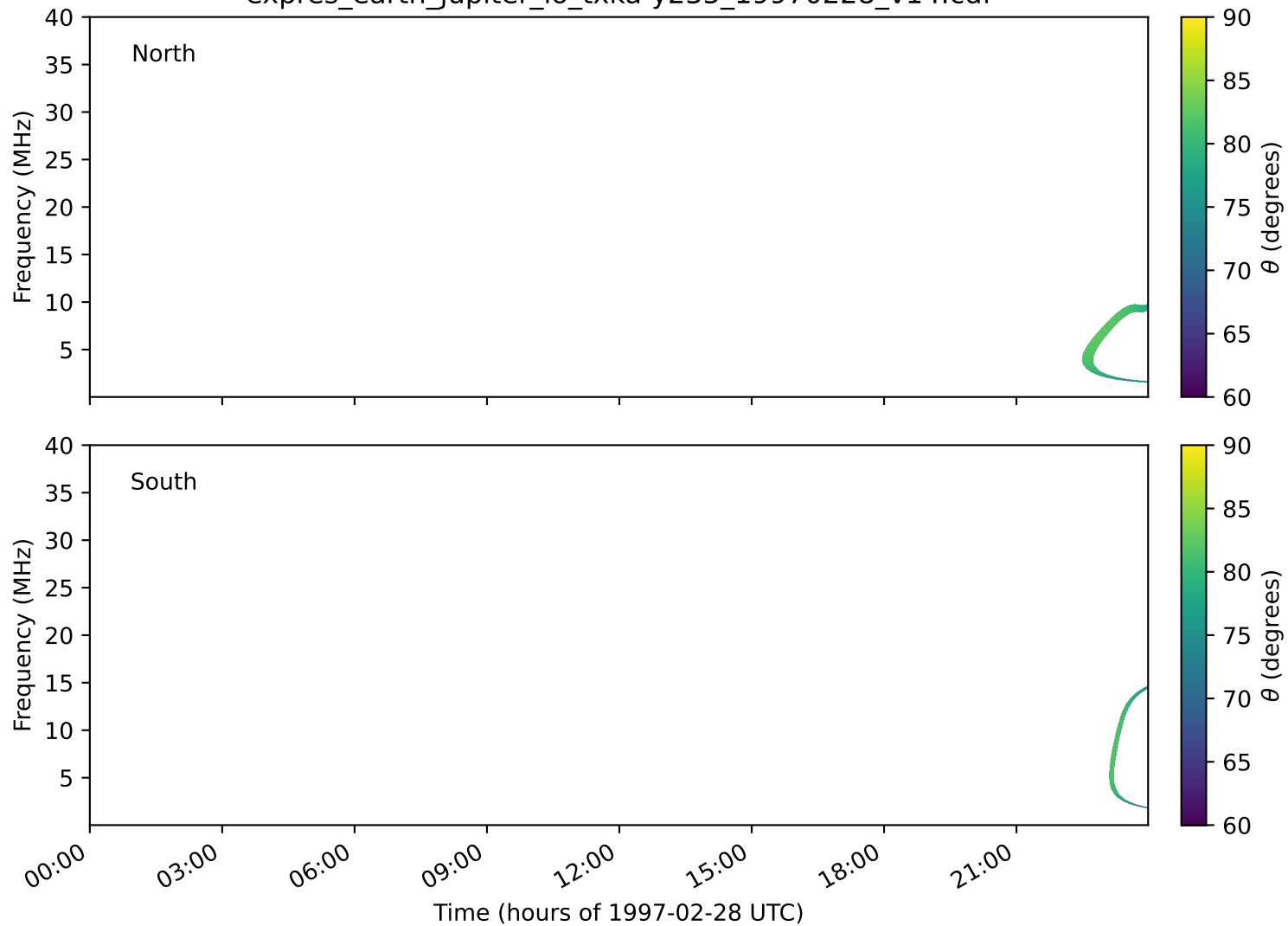
expres_earth_jupiter_io_txka-y235_19970228_v14.cdf
