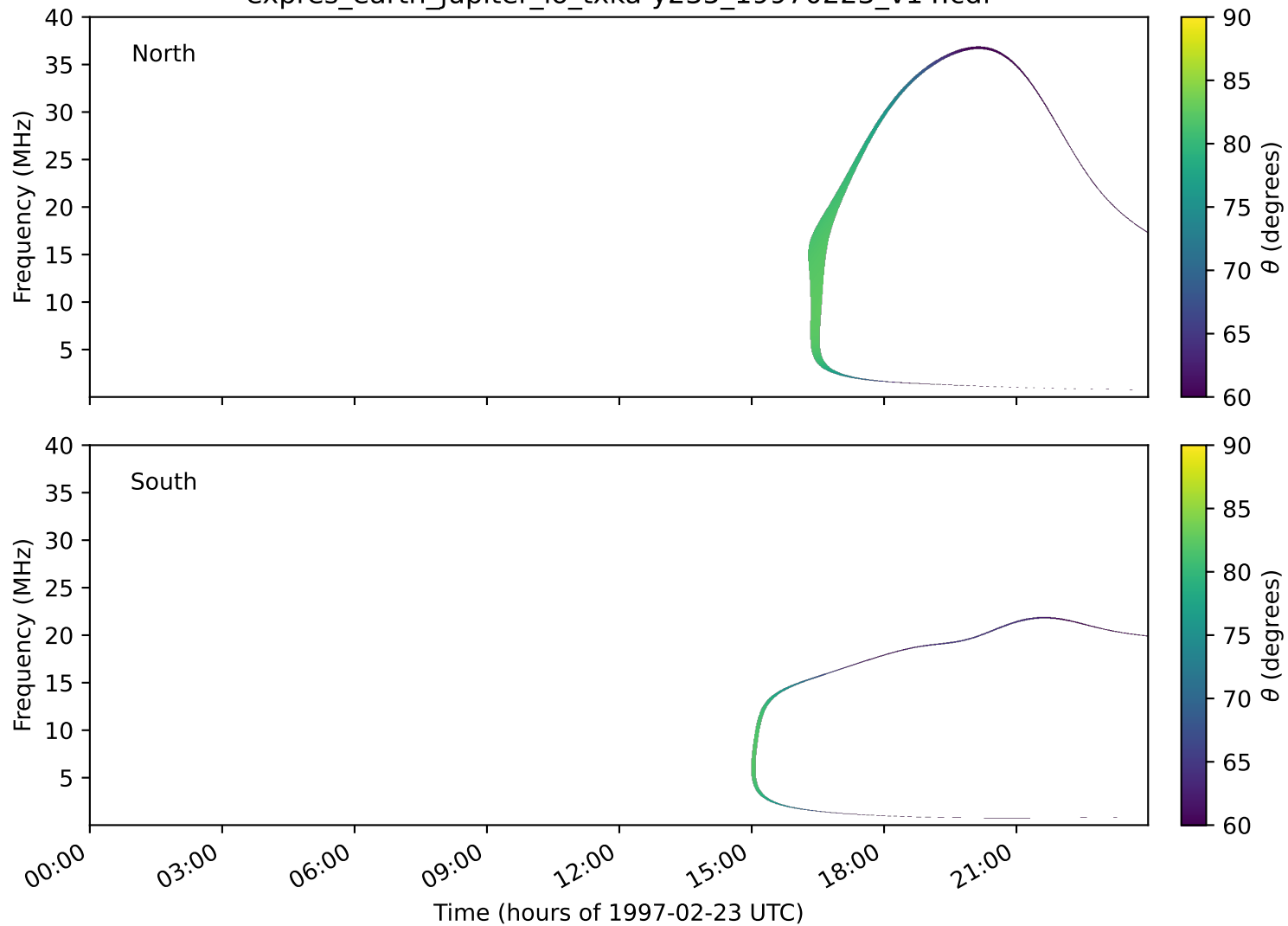
expres_earth_jupiter_io_txka-y235_19970223_v14.cdf
