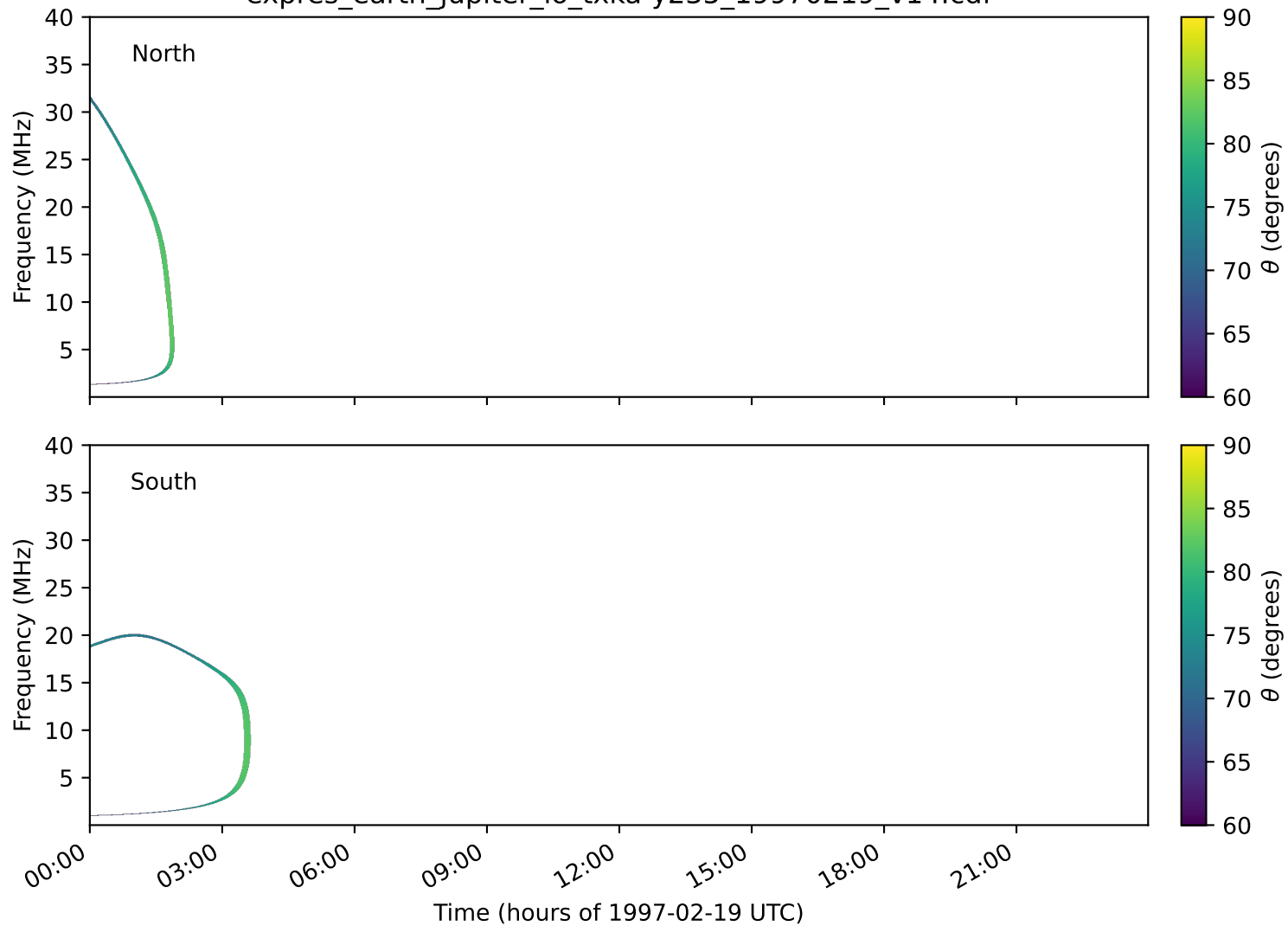
expres_earth_jupiter_io_txka-y235_19970219_v14.cdf
