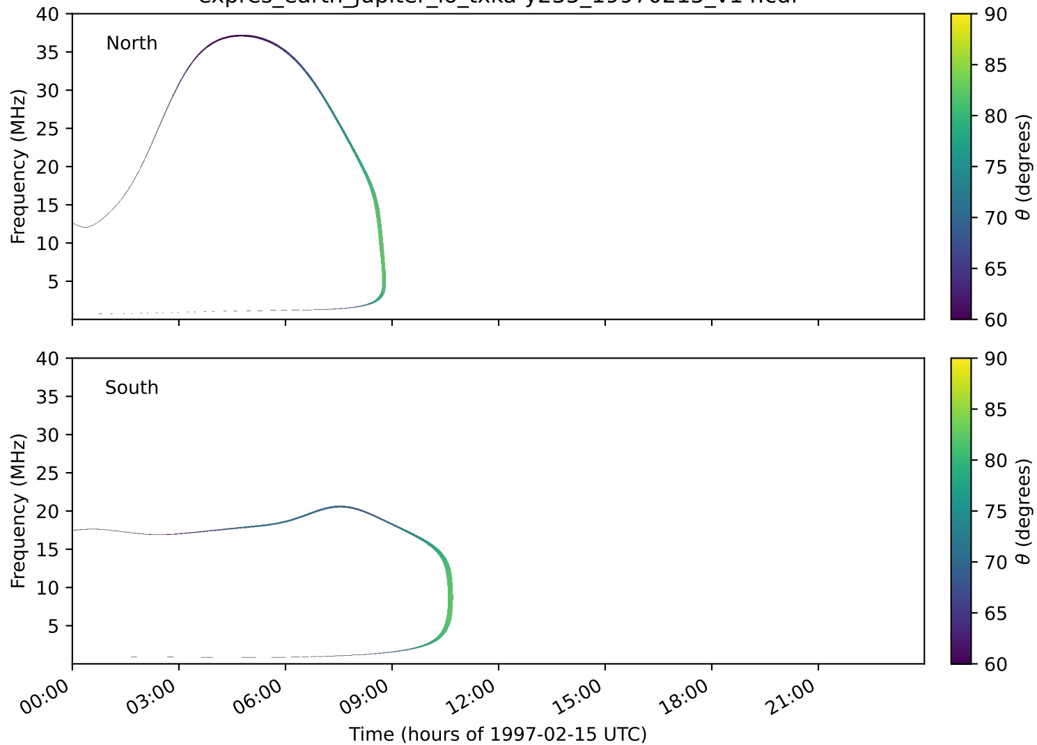
expres_earth_jupiter_io_txka-y235_19970215_v14.cdf
