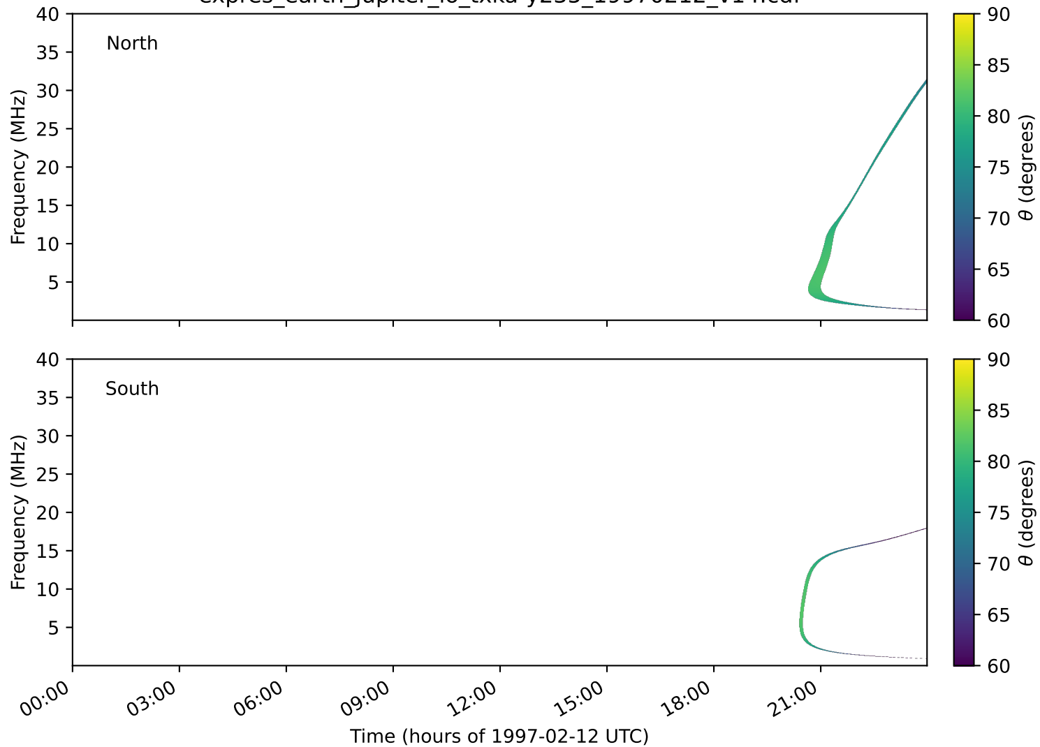
expres_earth_jupiter_io_txka-y235_19970212_v14.cdf
