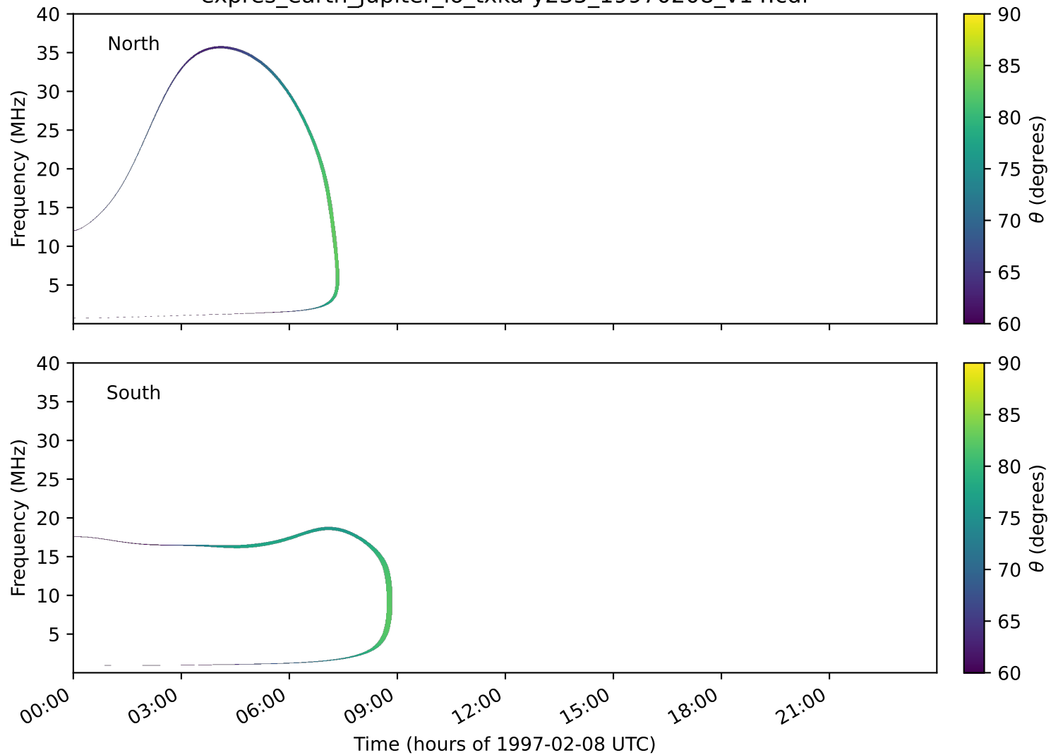
expres_earth_jupiter_io_txka-y235_19970208_v14.cdf
