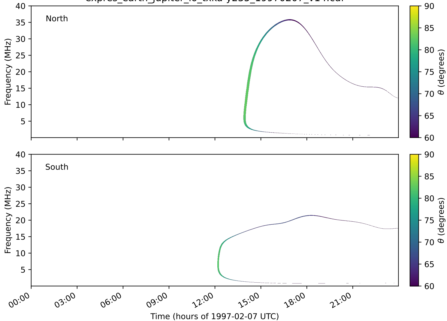
expres_earth_jupiter_io_txka-y235_19970207_v14.cdf
