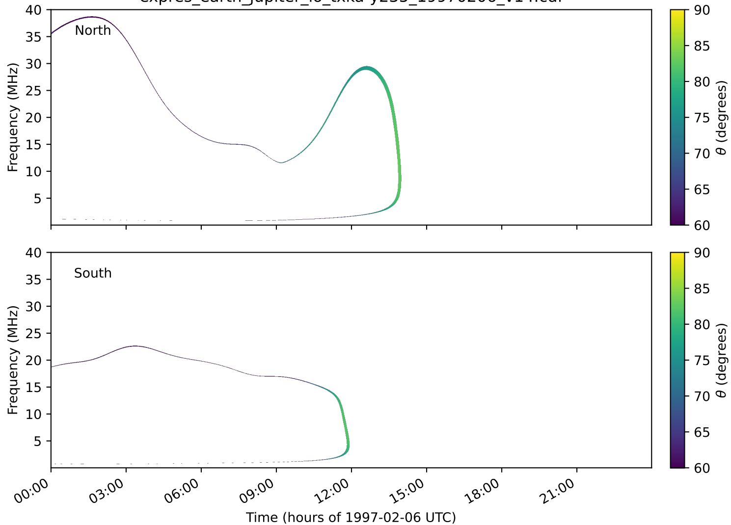
expres_earth_jupiter_io_txka-y235_19970206_v14.cdf
