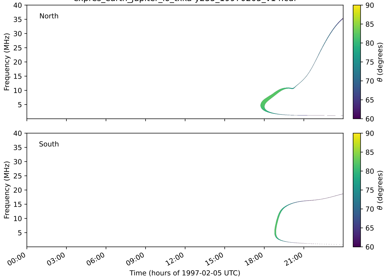
expres_earth_jupiter_io_txka-y235_19970205_v14.cdf
