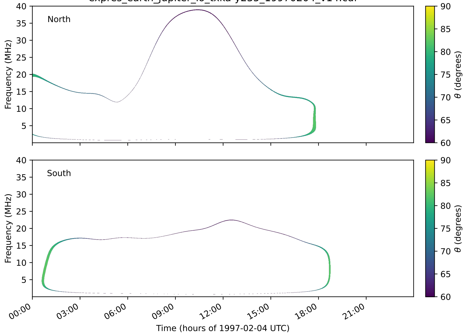
expres_earth_jupiter_io_txka-y235_19970204_v14.cdf
